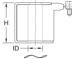
QT2 COIL
