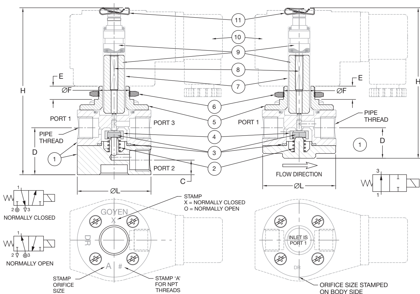
B6M3 CONSTRUCTION
