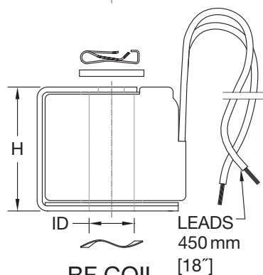
BF COIL
