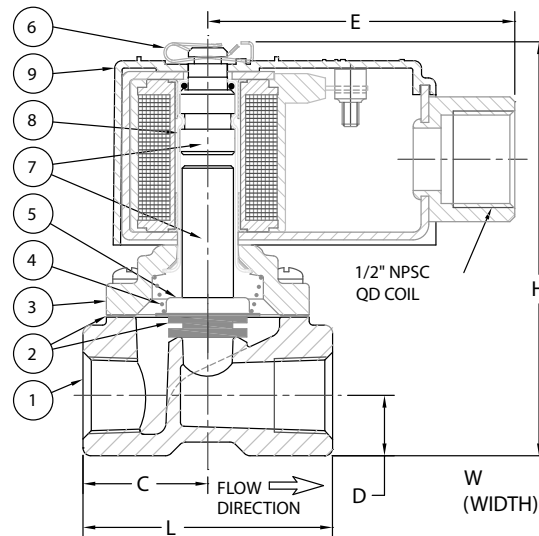
10QG CONSTRUCTION
