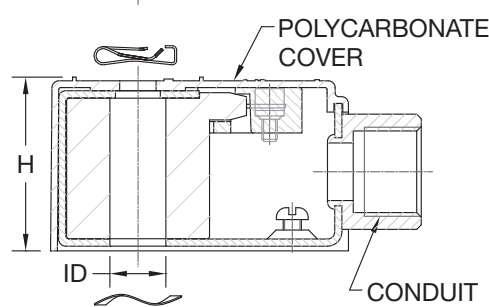
QD COIL
