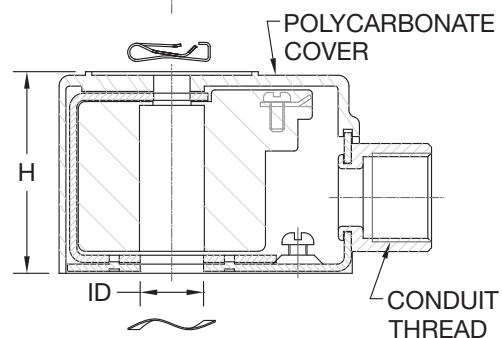
BD COIL
